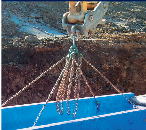
LIFTING CHAIN
